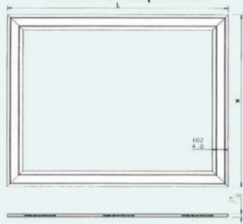
Reversible top frame
